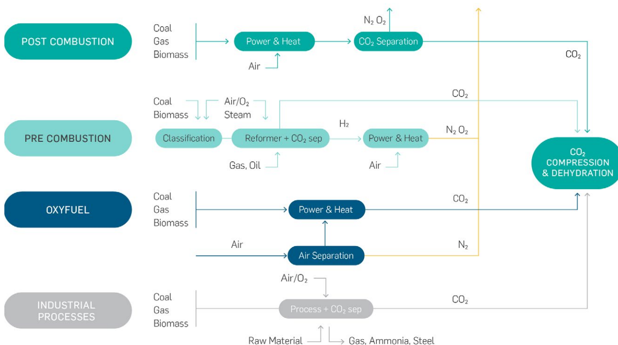
FIGURE 21 CARBON CAPTURE AND STORAGE PROCESS [REF. 101]
