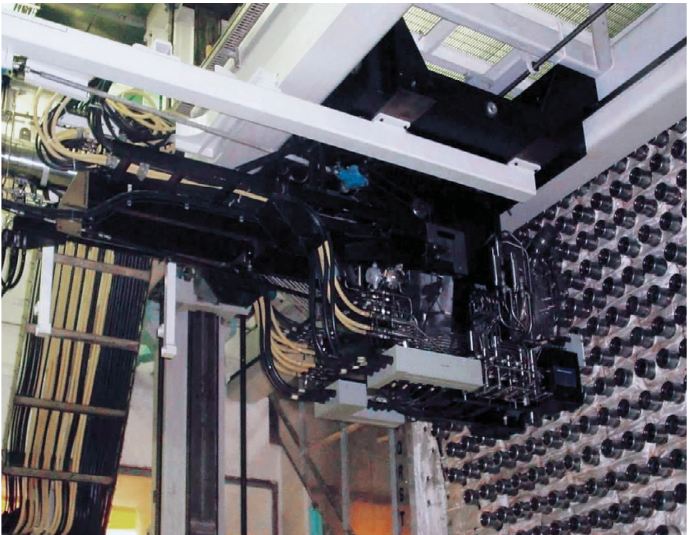
Fuelling Machine
