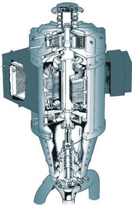
Heat Transport Pump and Motor
