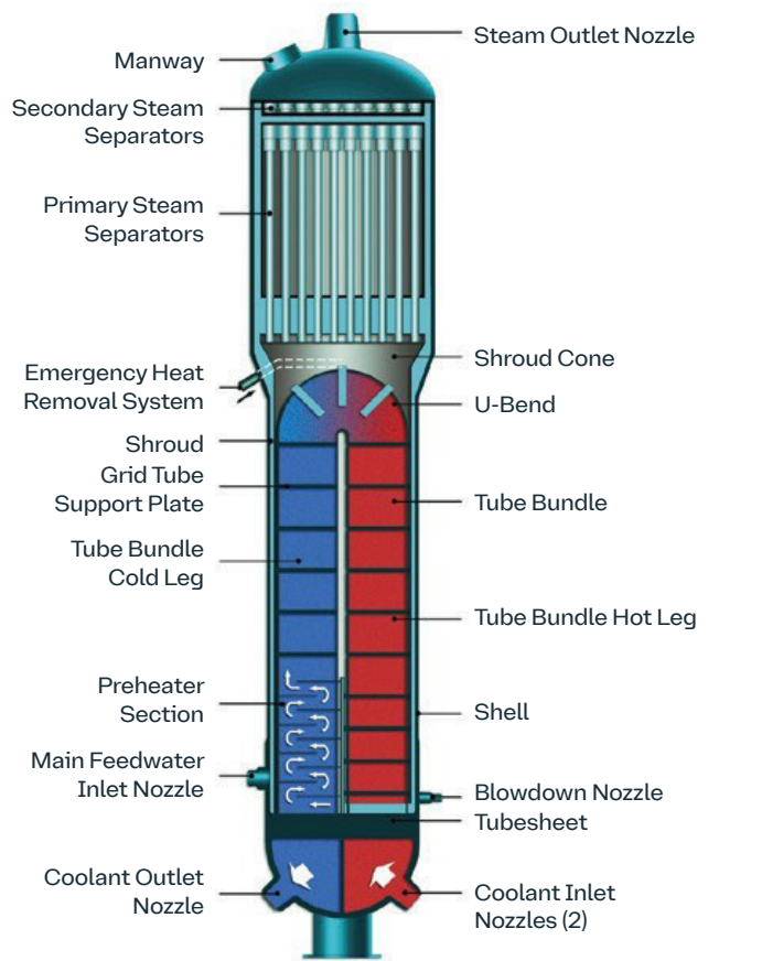
Steam Generator
