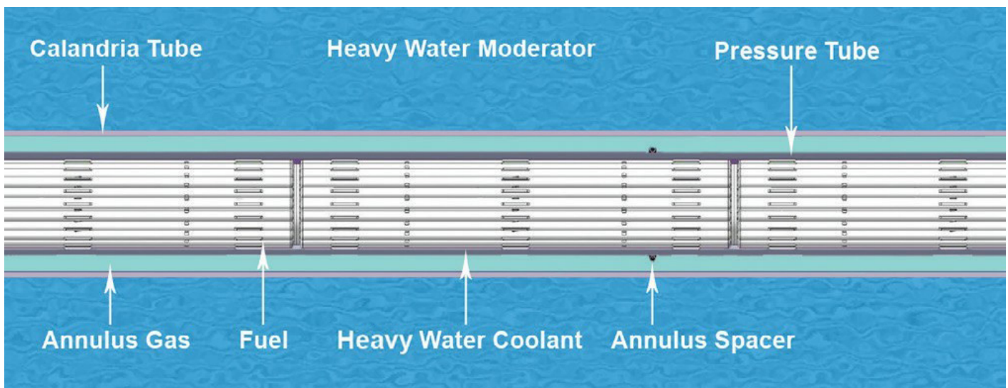
Fuel Channel Assembly
