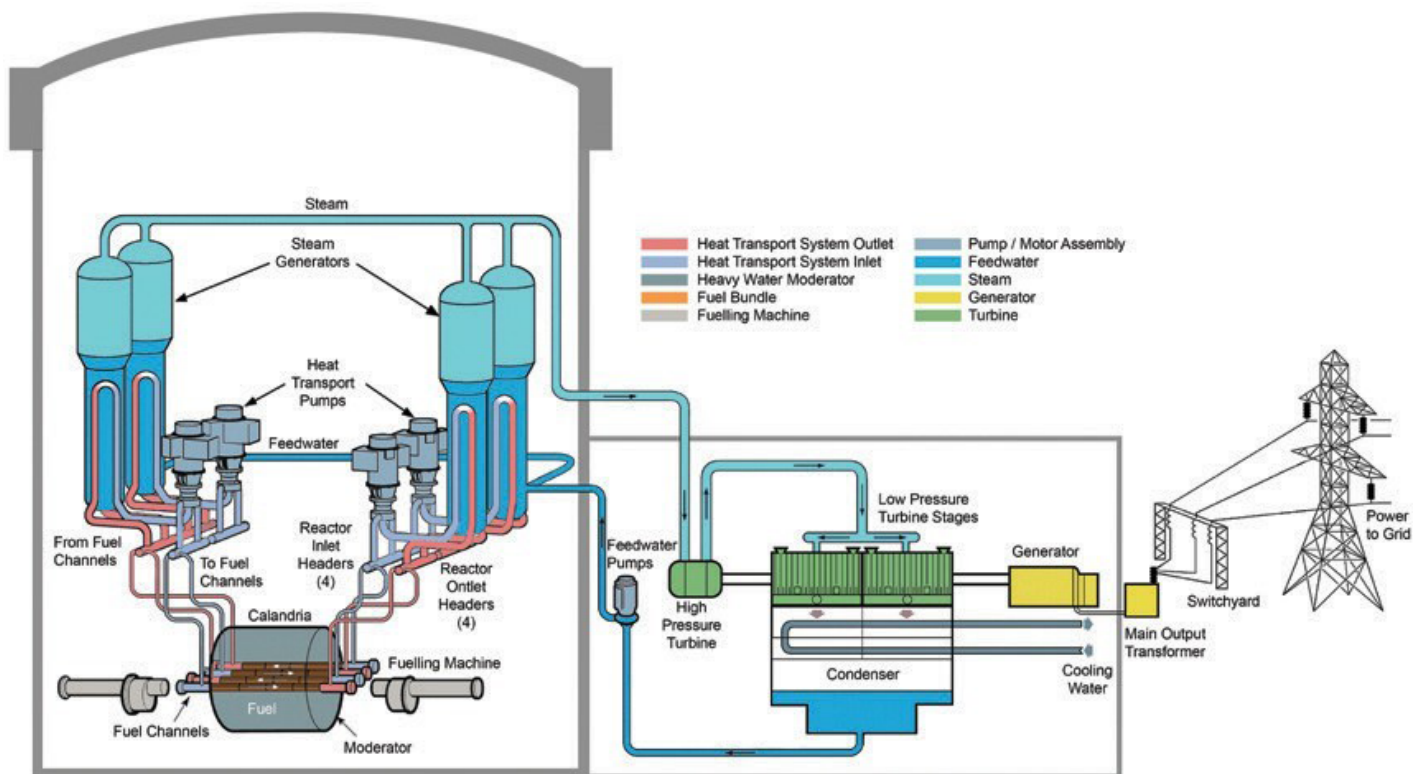
Overall Plant Flow Diagram
