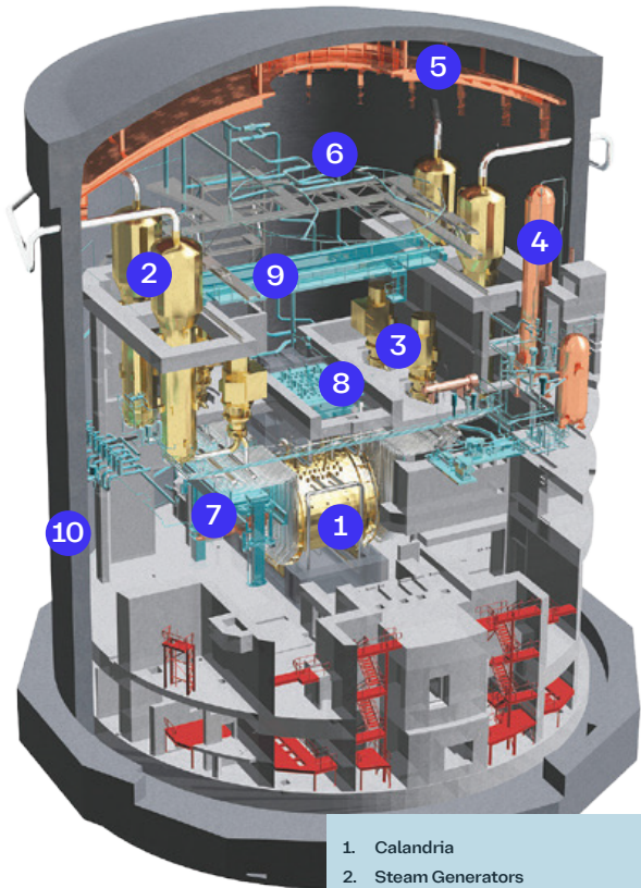
Reactor Assembly
